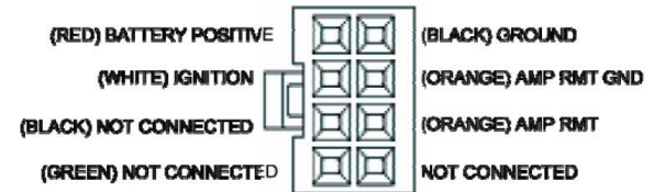
Figure 1.3, power connector diagram
