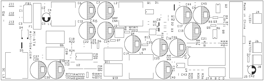
M1-ATX, top view
